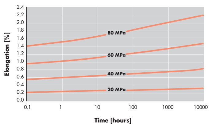
Creep curves Grivory HT2V-5H at 80°C
